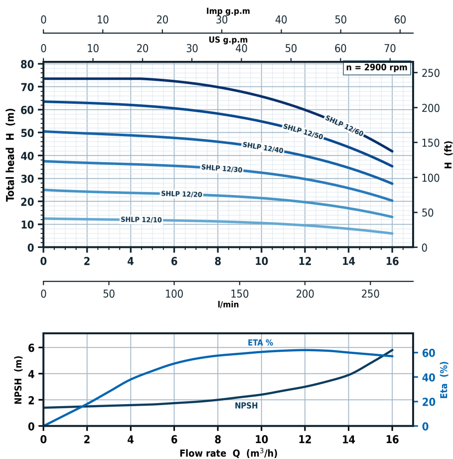
PERFORMANCE CHART AT n=2900 RPM
